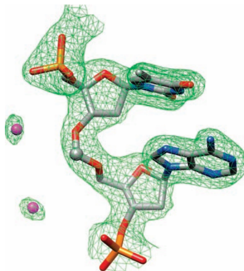
Figure 1. Quality of the electron density. Final Fourier sum 2F_o - F_c electron density ( 1\sigma threshold) around the T4 \mathbf{fA5} dimer is shown as a green meshwork and water molecules are shown as magenta spheres.
