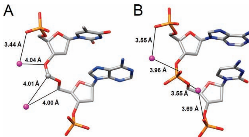
Figure 4. Comparison of water molecules associated with the backbones of (A) formacetal linkage in T4fA5 and (B) phosphate linkage in A7pC8. Contacts between water molecules associated with the formacetal and phosphate moiety in the structures of the chemically modified and native decamers, respectively, are shown with thin lines and distances in Å.
