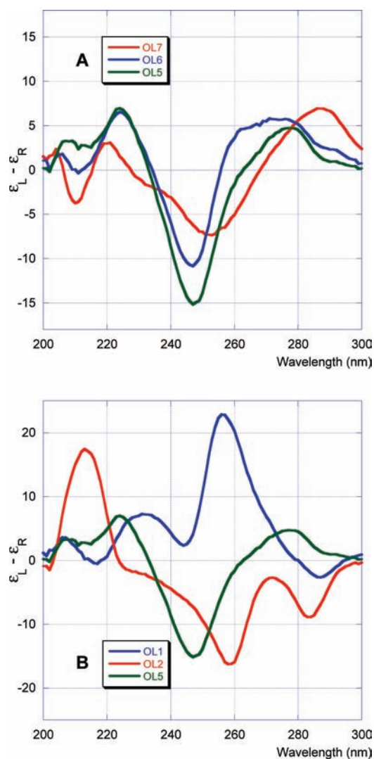
Figure 5. CD spectra of oligonucleotides.
