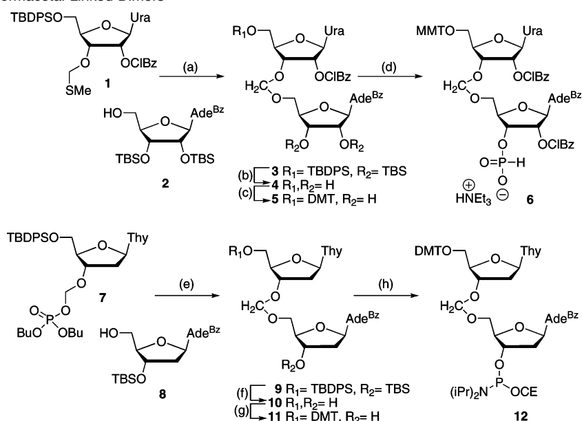
Scheme 1. Synthesis of Formacetal Linked Dimers a
