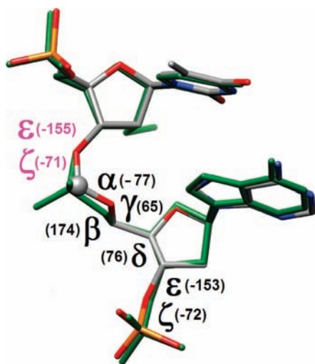
Figure 3. Overlay of the T4fA5 and U_{Mc}6pA7 (green bonds) dinucleotides. Torsion angles of the formacetal linkage are depicted in black. Values of the \epsilon and \zeta torsion angles in the 5'-flanking T4 residue are highlighted in purple.
