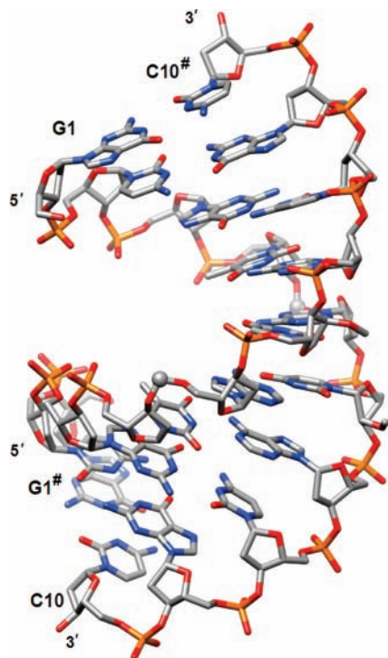
Figure 2. Crystal structure of the duplex [d(GCGTfAU_{Mc}ACGC)]_2 ( OL7 ). The formacetal carbon is highlighted with a sphere and the hash symbol indicates a symmetry-related strand. The view is across the major (top) and minor grooves (bottom).
